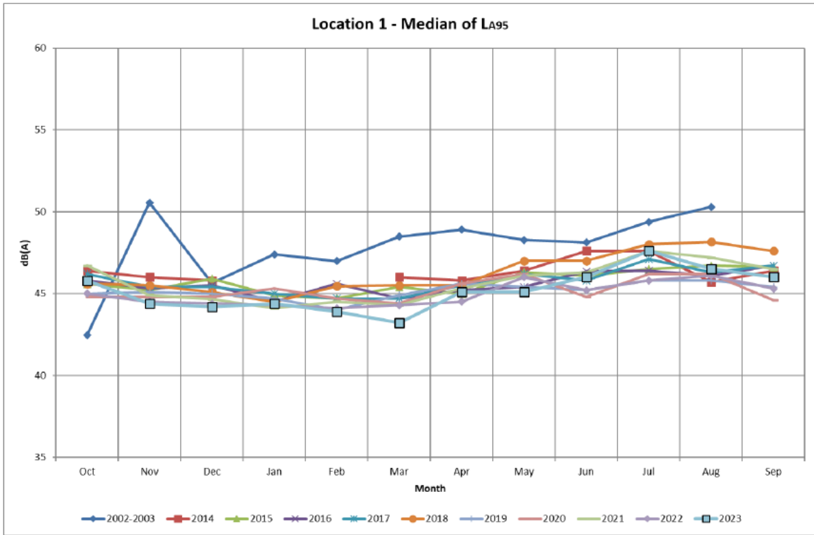
Figure 6-2 Comparison of noise levels measured at Location 1 (North Monitor) for base period (2002 – 2003) and 2014 – 2023.
