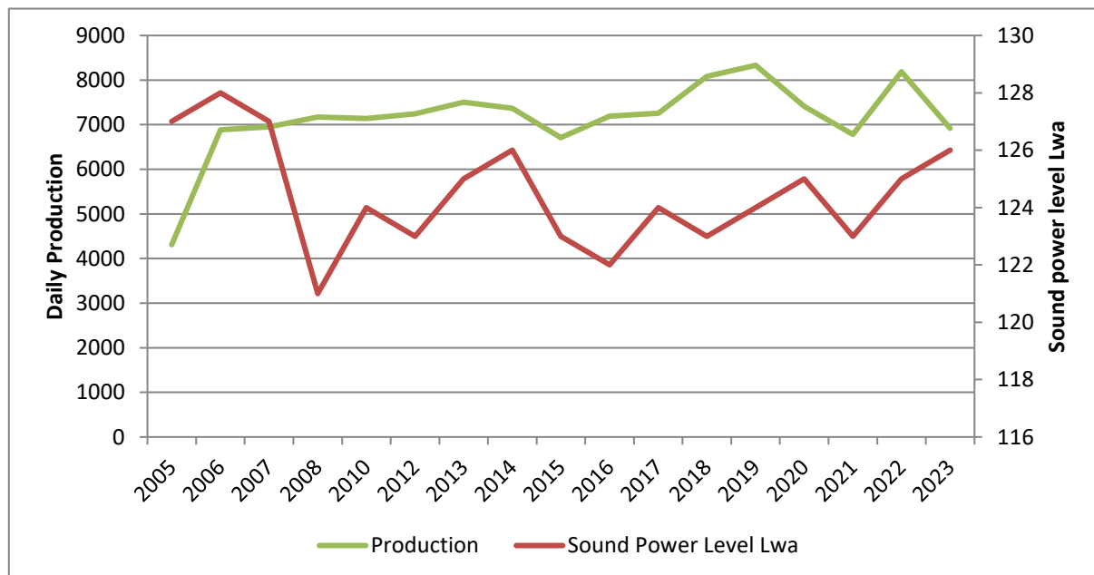
Figure 6-1 Summary of Wagerup sound power levels 20 location abbreviated method from 2005 to 2023
