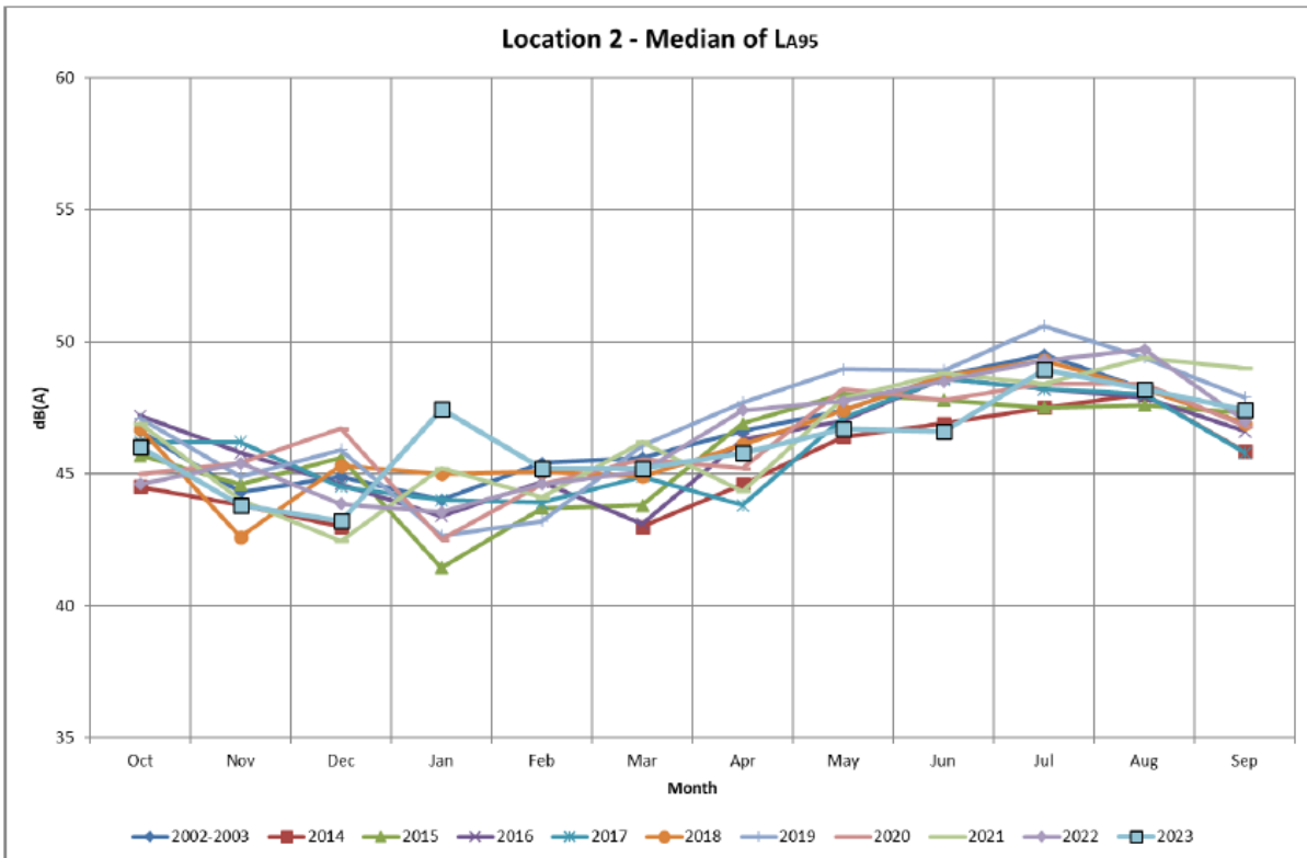
Figure 6-3 Comparison of noise levels measured at Location 2 (South Monitor) for base period (2002 – 2003) and 2014 – 2023.
